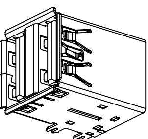
Mating Drawing
