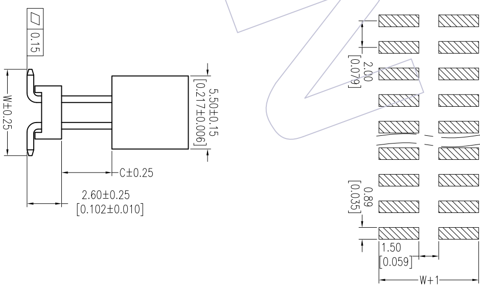
Recommended P.C.B Layout(Top Side) (PCB BOARD TOLERANCE±0.05)
