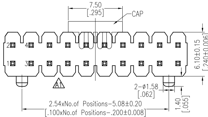
Dual Numbers
